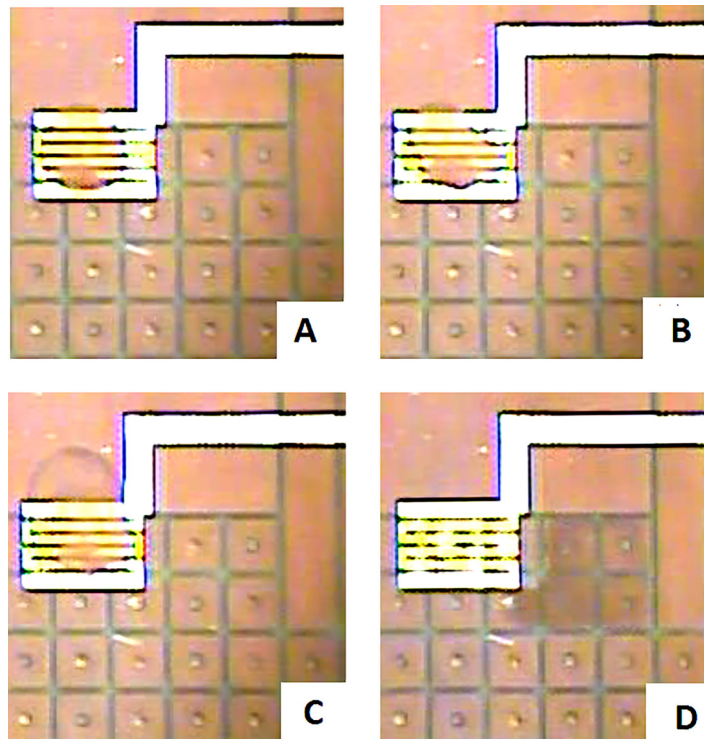
FIG. 13. (a) A 2\times sized droplet containing E. coli , sitting on top of the electroporation electrode before a double pulse. (b) The 2\times droplet sitting on top of the electroporation electrode, immediately after a double pulse. (c) A 6\times droplet formed from the 4\times recovery droplet merged with the 2\times sample droplet. (d) The 6\times recovered droplet being transported off the electroporation electrode.
